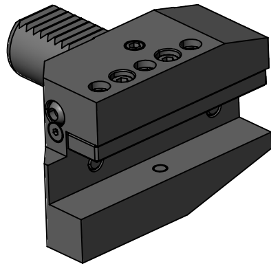
90DEG VDI30 STATIC TOOL OUTPUT: 3/4" SQR SHANK COOLANT: EXTERNAL
